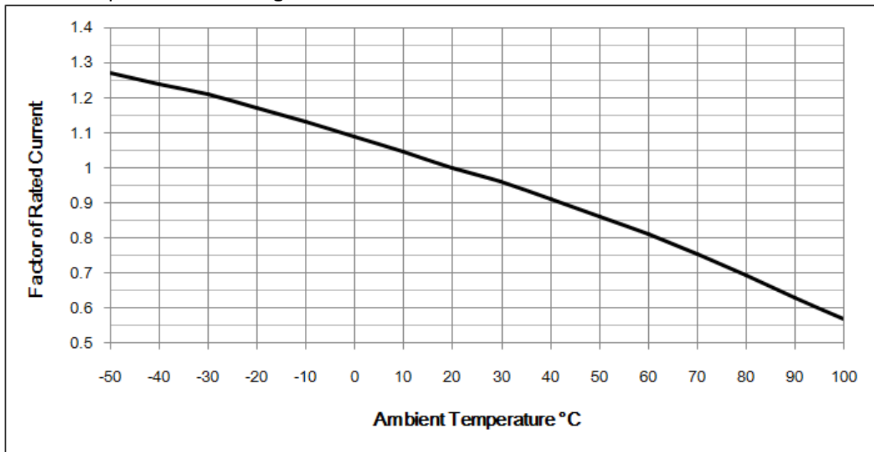
Temperature Re-Rating Curve
